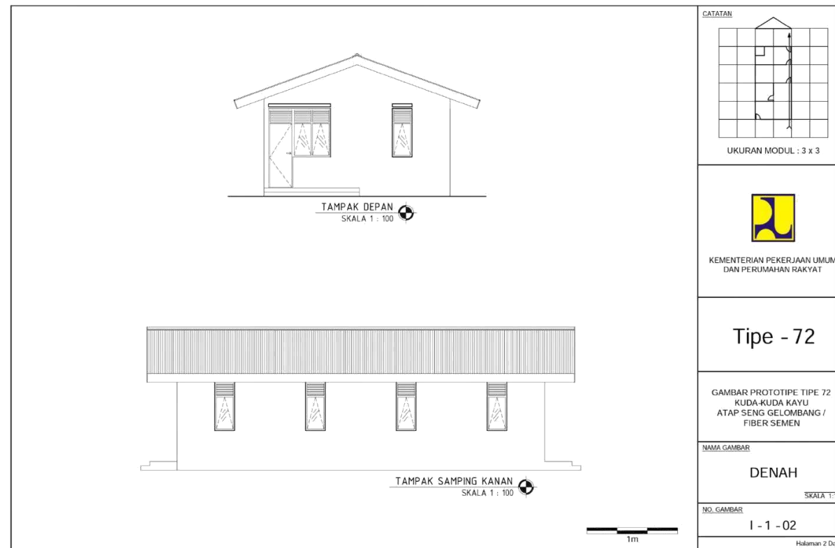
Gambar II.448. Tipe 72 Tampak I-1-02
