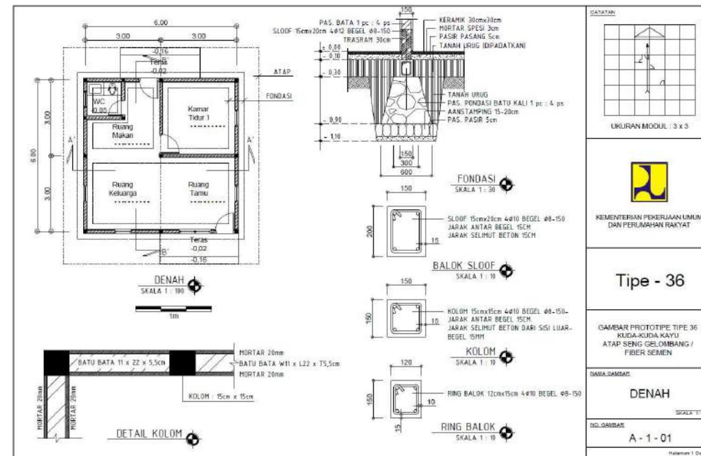
Gambar II.422. Tipe 36 Denah A-1-01
