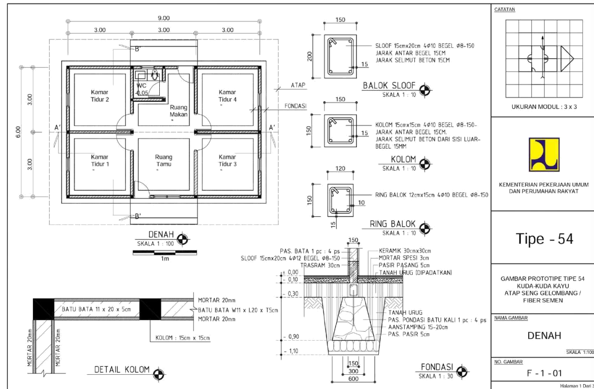
Gambar II.437. Tipe 54 Denah F-1-01
