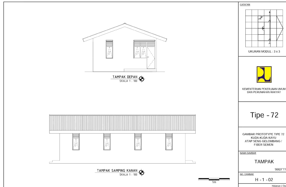
Gambar II.444. Tipe 72 Tampak H-1-02
